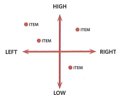
Figure 5.14 2x2 matrix.
